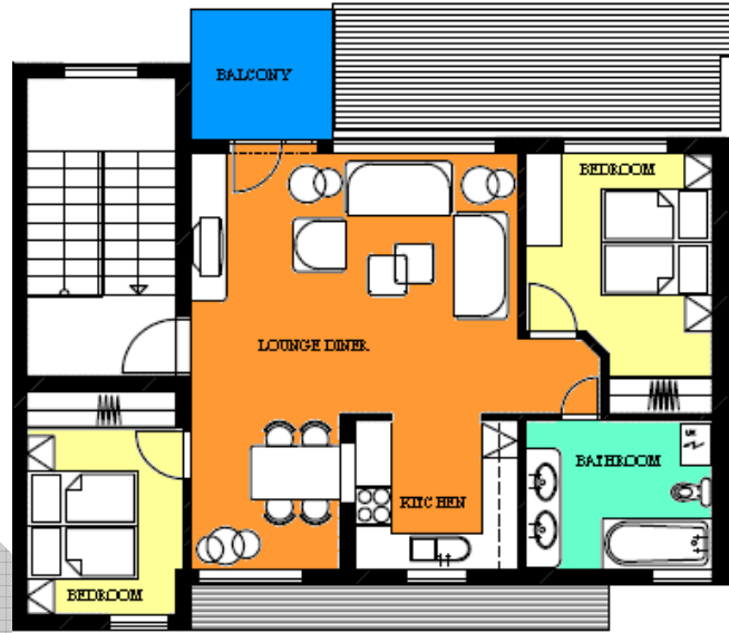
Floor Plan two bedroom apartment No.203
