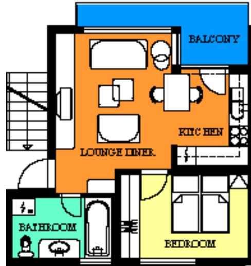
Floor Plan one bedroom apartment No.102
