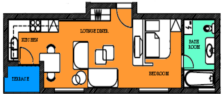
Floor Plan one bedroom studio apartment No. 106
