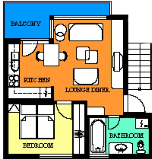
Floor Plan one bedroom apartment No. 101
